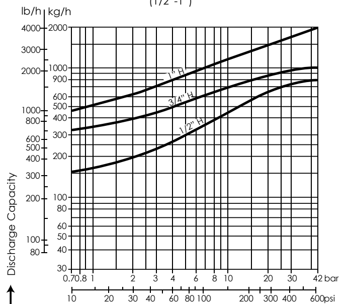
Discharge Capacities (1/2"-1")
